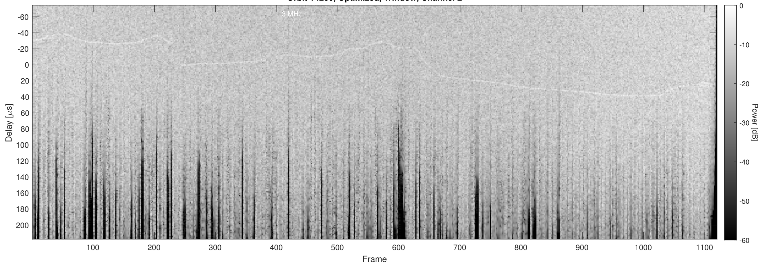
Orbit 14266, Optimized, Window, Channel 2
