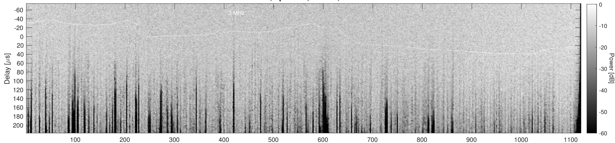
Orbit 14266, Cluttergram
