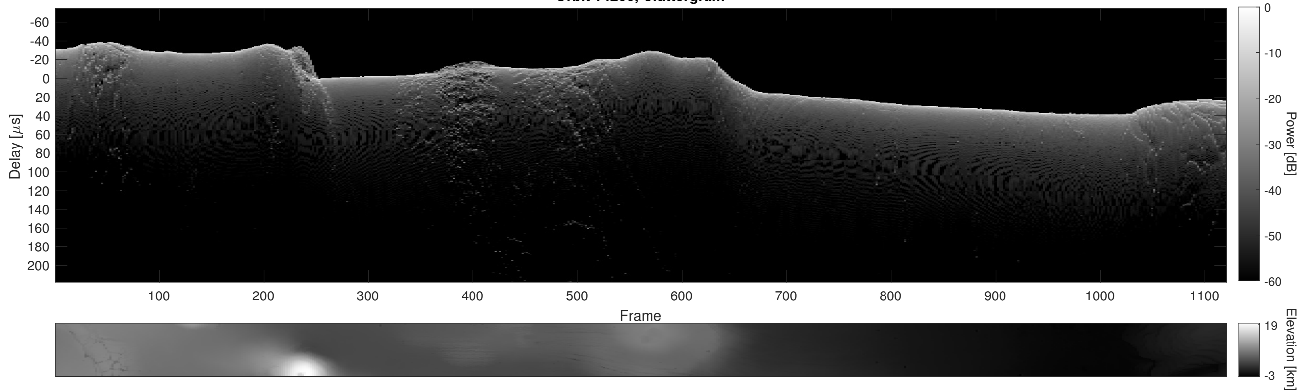
Orbit 14266, Cluttergram
