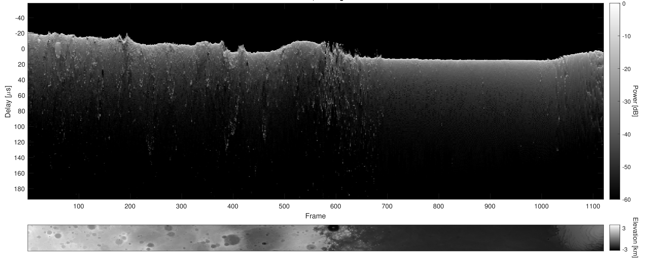
Orbit 14268, Cluttergram
