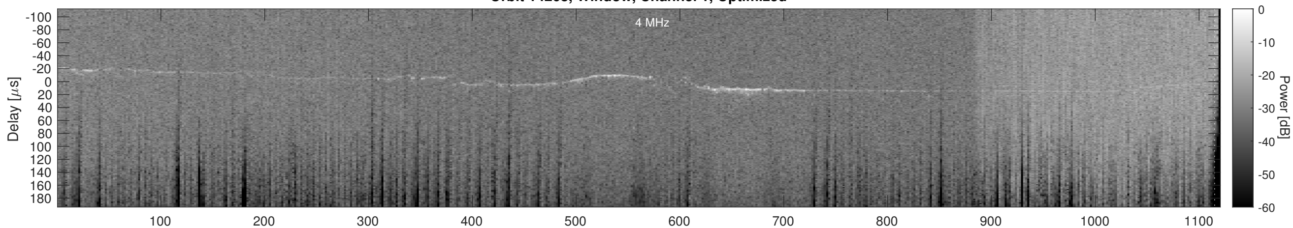
Orbit 14268, Cluttergram
