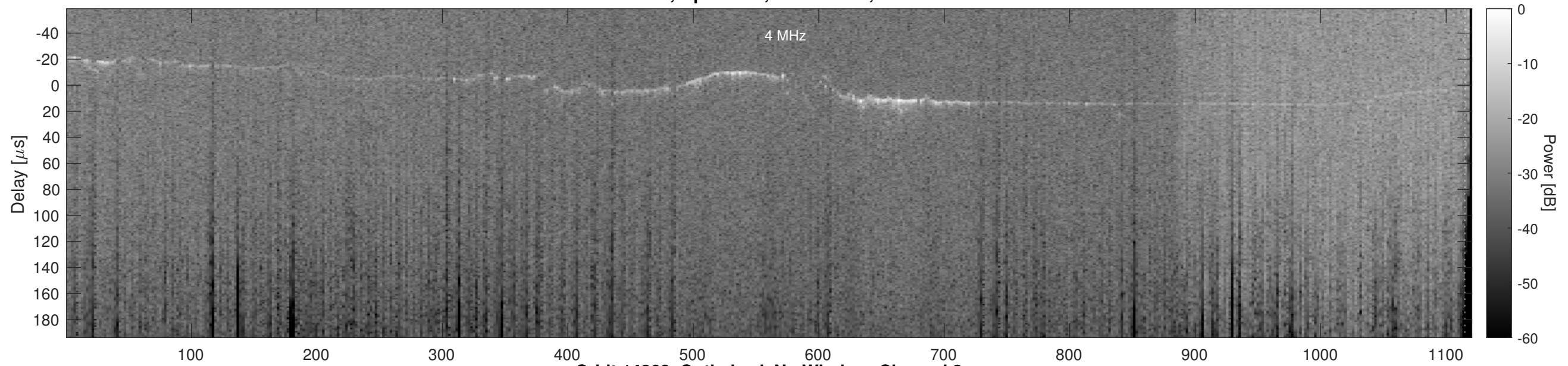
Orbit 14268, Optimized, No Window, Channel 2
