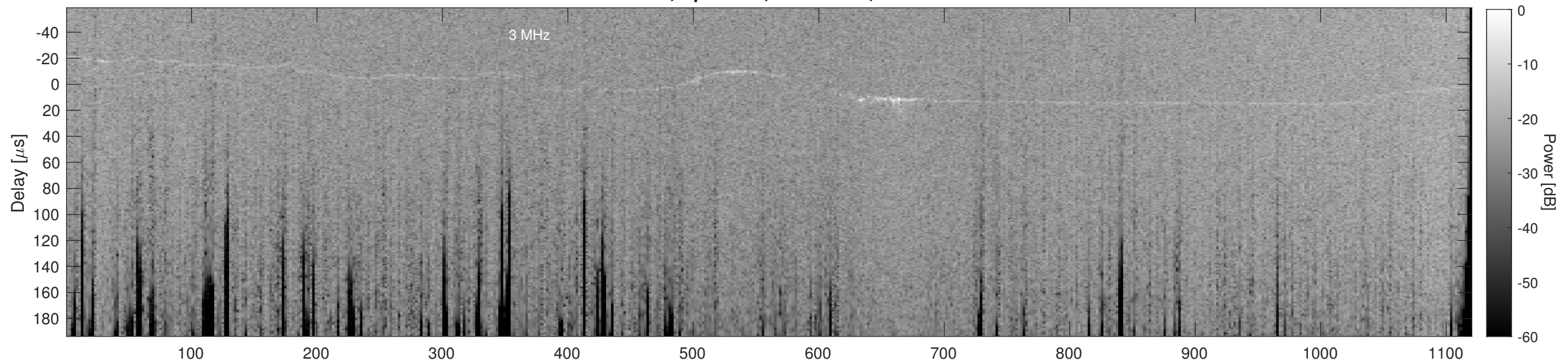
Orbit 14268, Cluttergram
