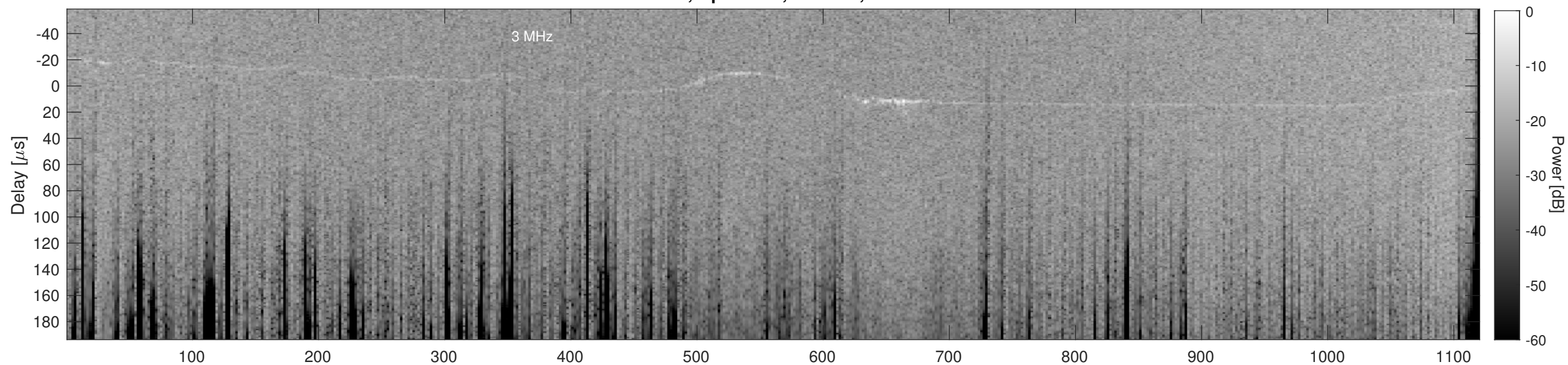
Orbit 14268, Cluttergram
