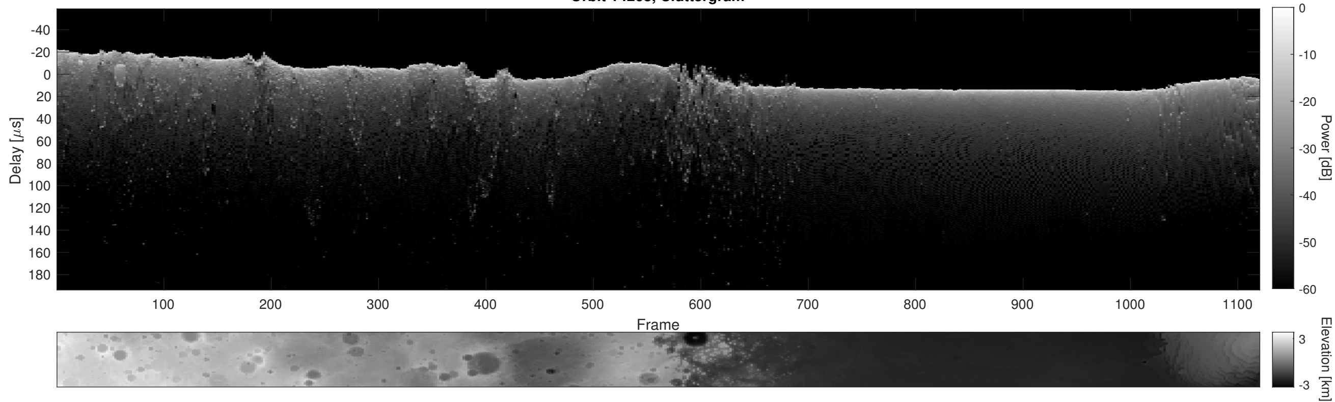
Orbit 14268, Cluttergram
