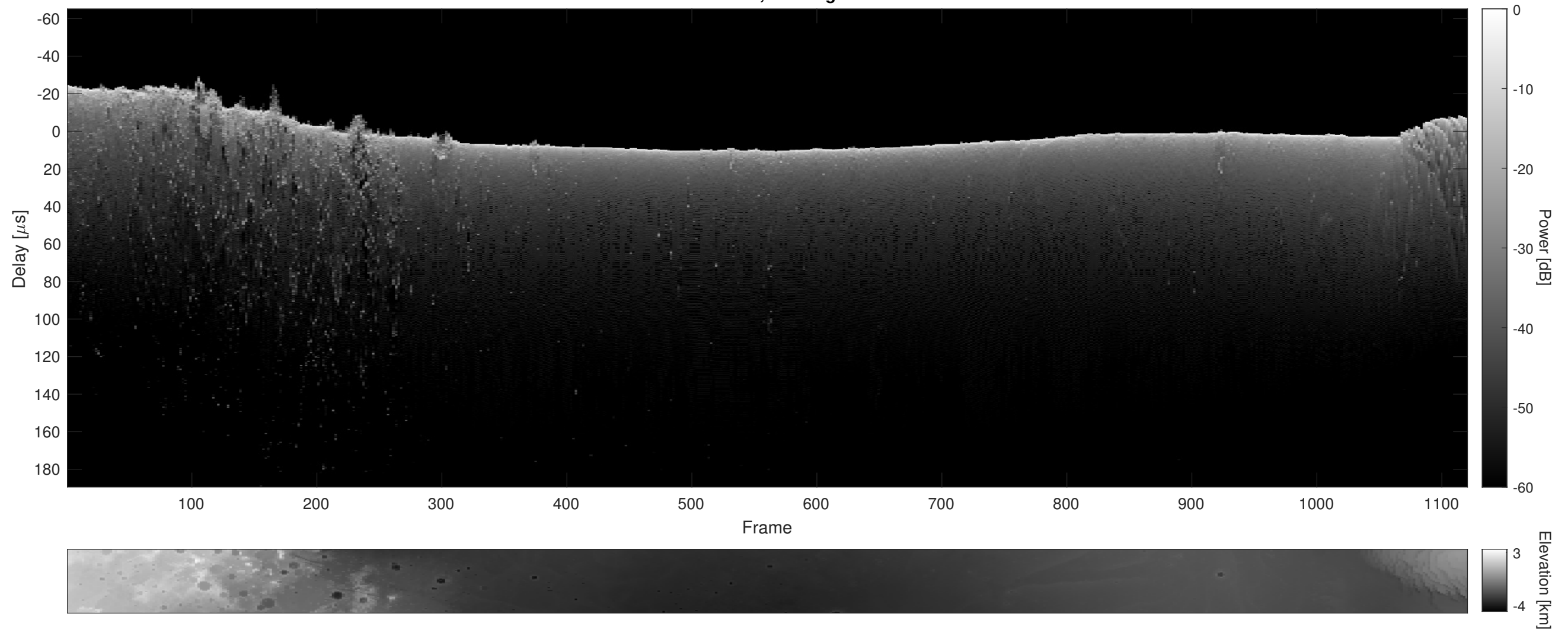
Orbit 14271, Cluttergram
