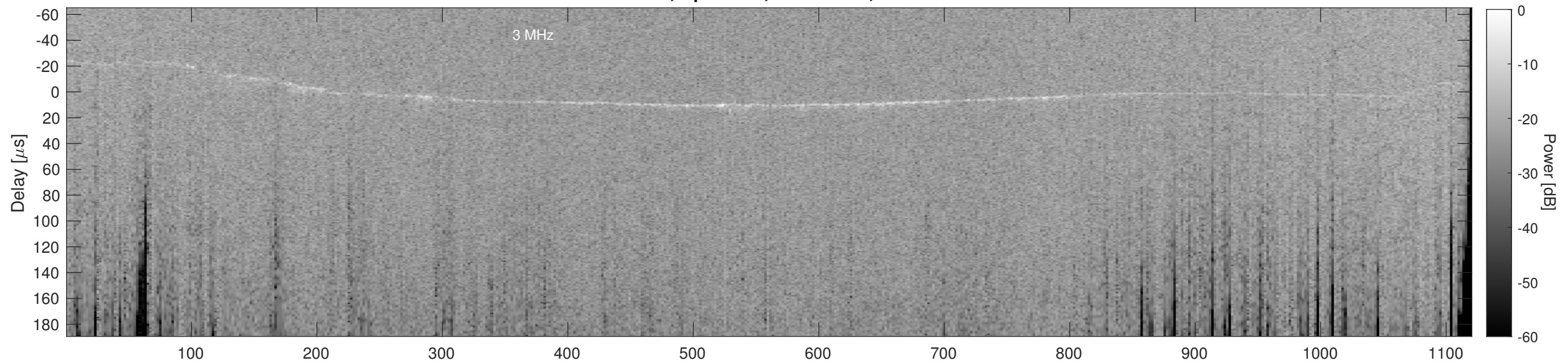
Orbit 14271, Cluttergram
