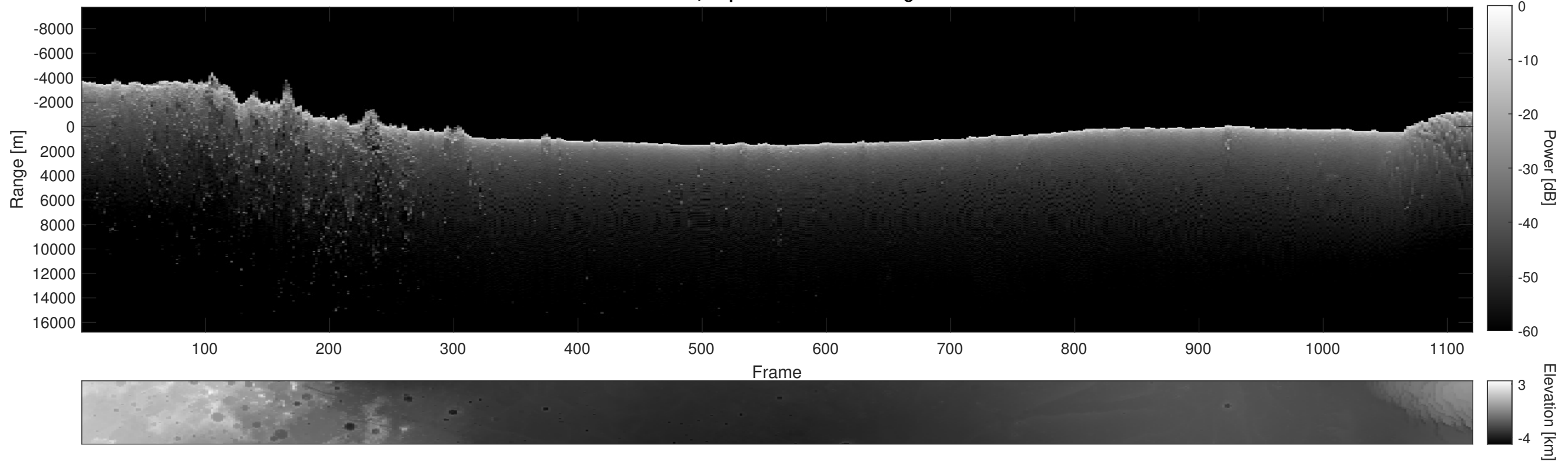
Orbit 14271, Depth-Corrected Cluttergram
