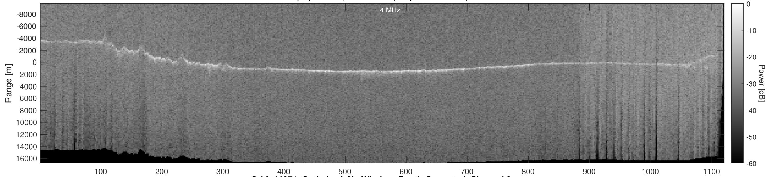
Orbit 14271, Optimized, No Window, Depth-Corrected, Channel 2
