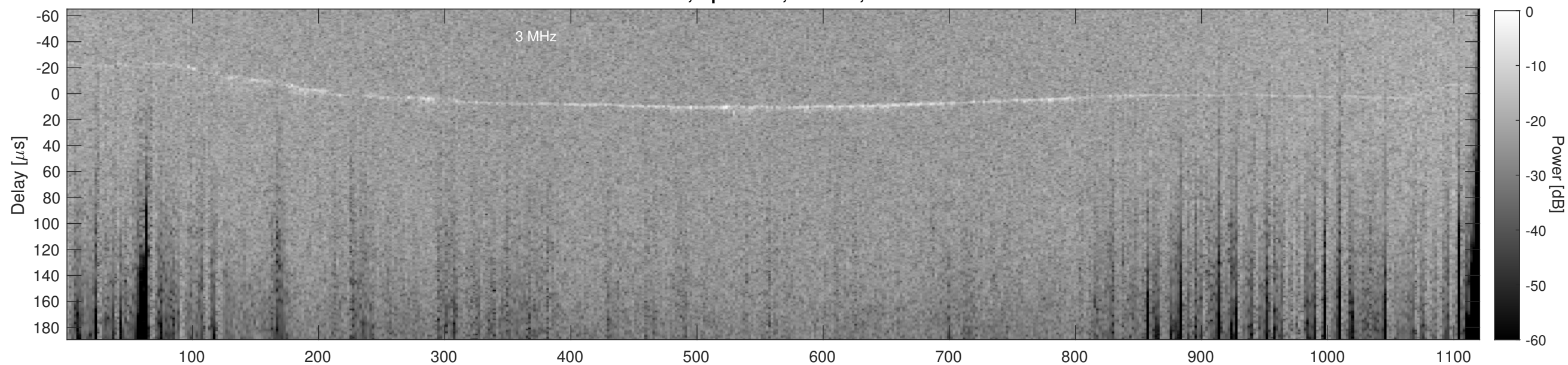
Orbit 14271, Cluttergram
