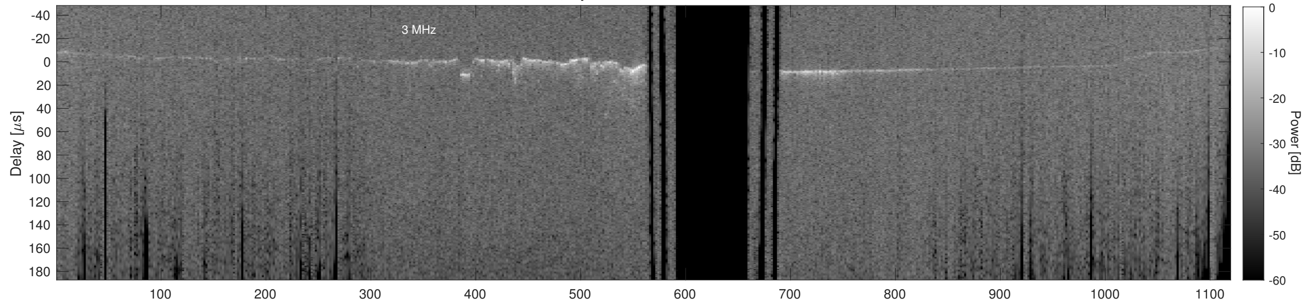
Orbit 14272, Cluttergram
