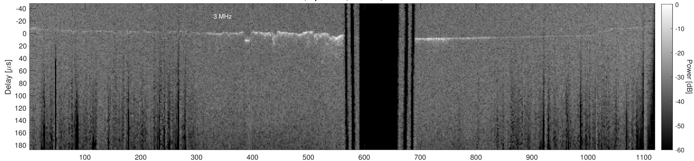
Orbit 14272, Cluttergram
