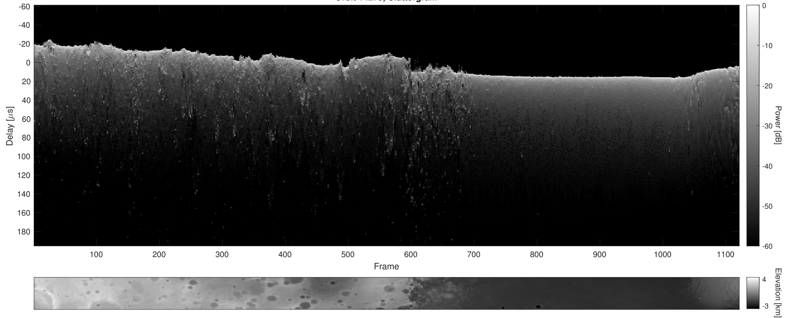
Orbit 14275, Cluttergram
