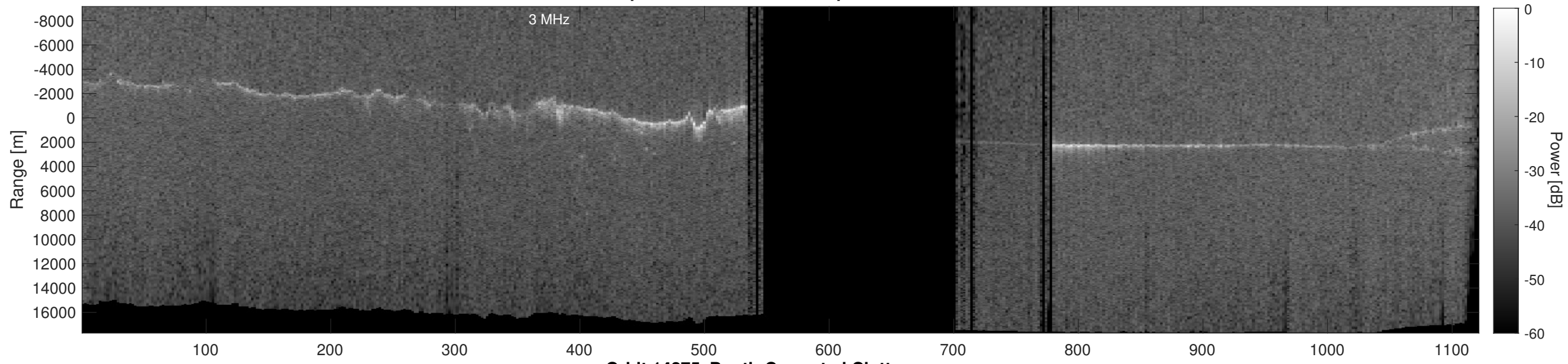
Orbit 14275, Depth-Corrected Cluttergram
