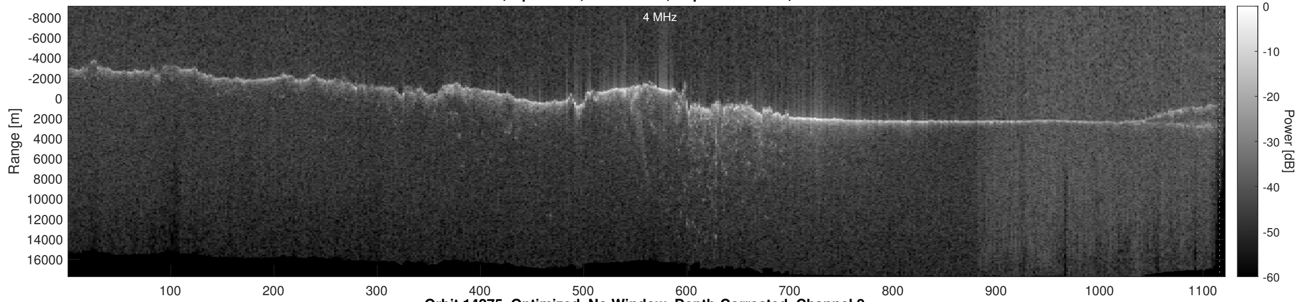
Orbit 14275, Optimized, No Window, Depth-Corrected, Channel 2
