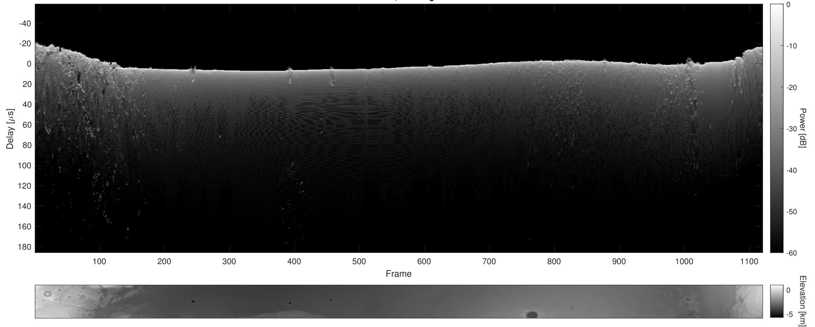
Orbit 14277, Cluttergram
