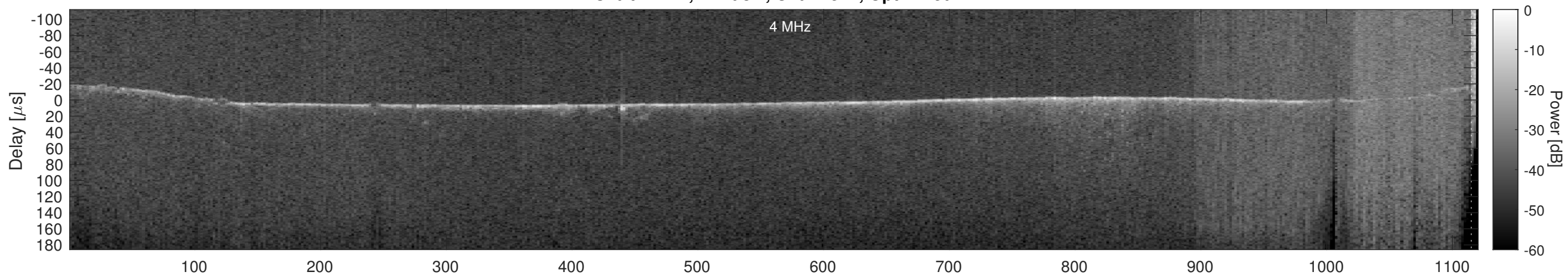
Orbit 14277, Cluttergram
