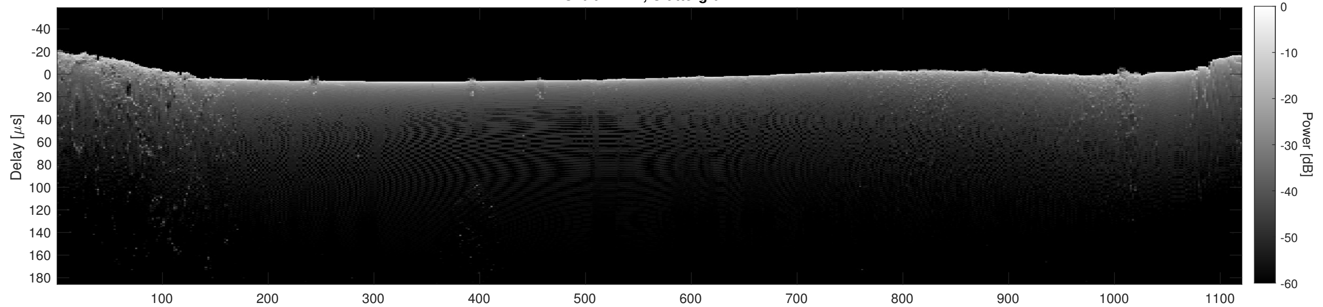
Orbit 14277, Cluttergram
