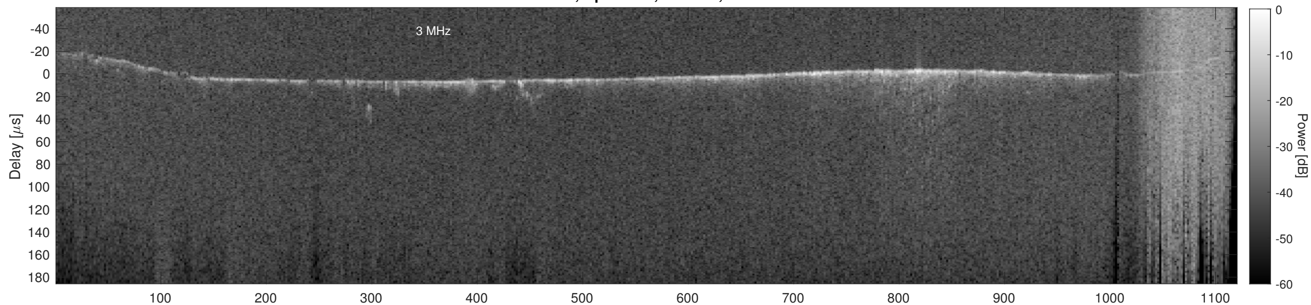
Orbit 14277, Cluttergram
