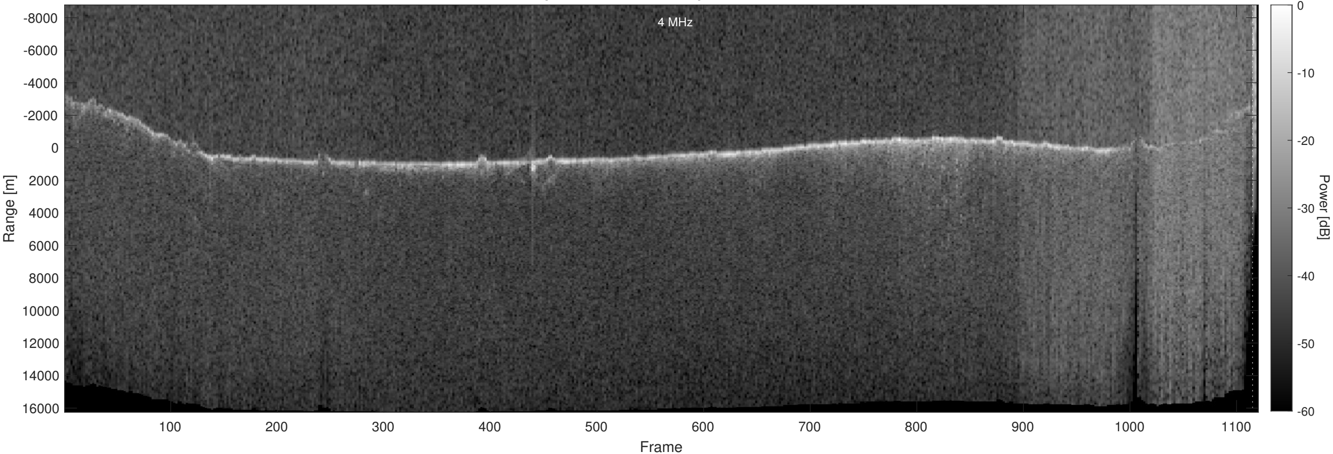
Orbit 14277, Optimized, Window, Depth-Corrected, Channel 2
