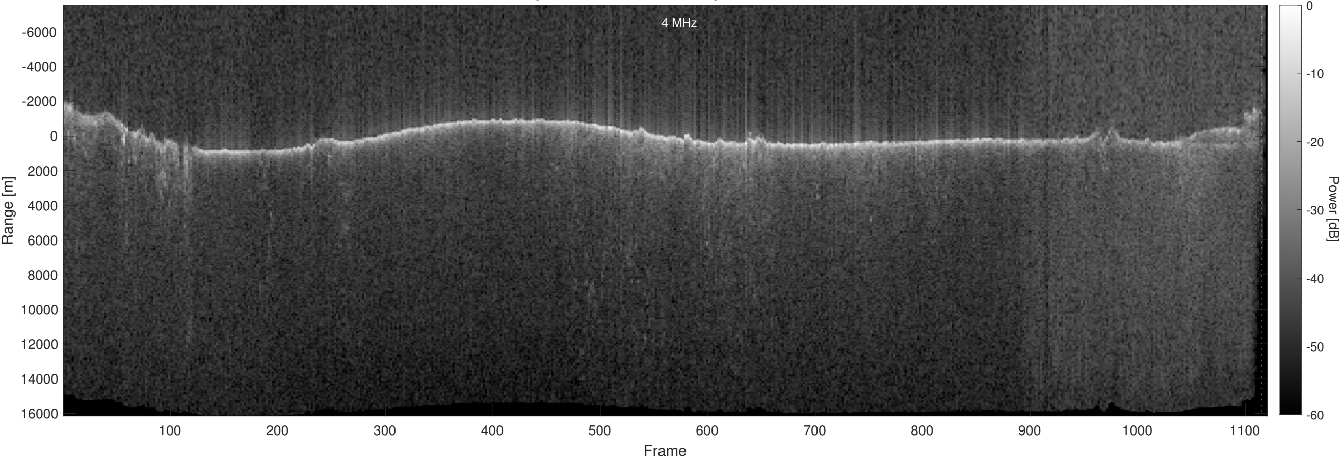
Orbit 14281, Optimized, No Window, Depth-Corrected, Channel 2
