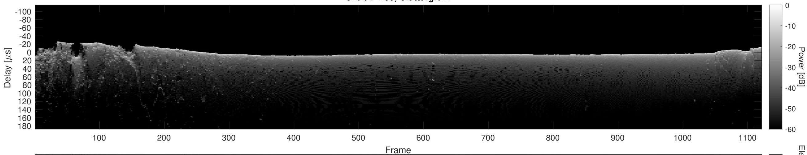
Orbit 14283, Cluttergram
