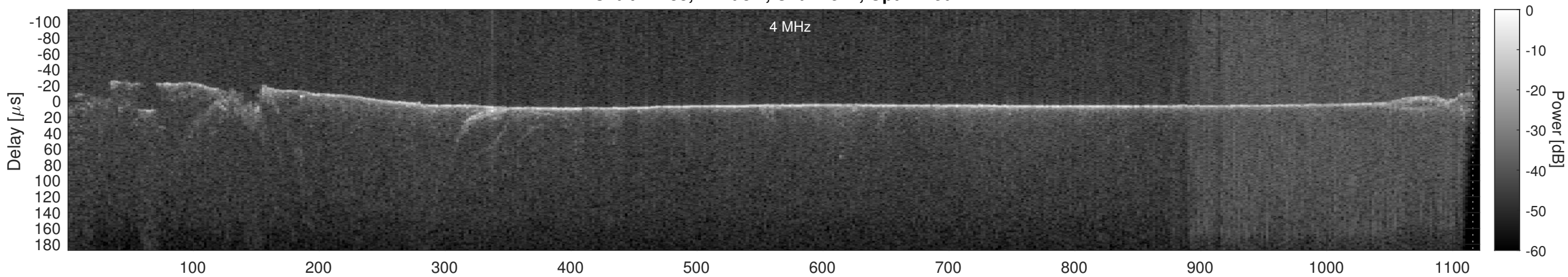
Orbit 14283, Cluttergram
