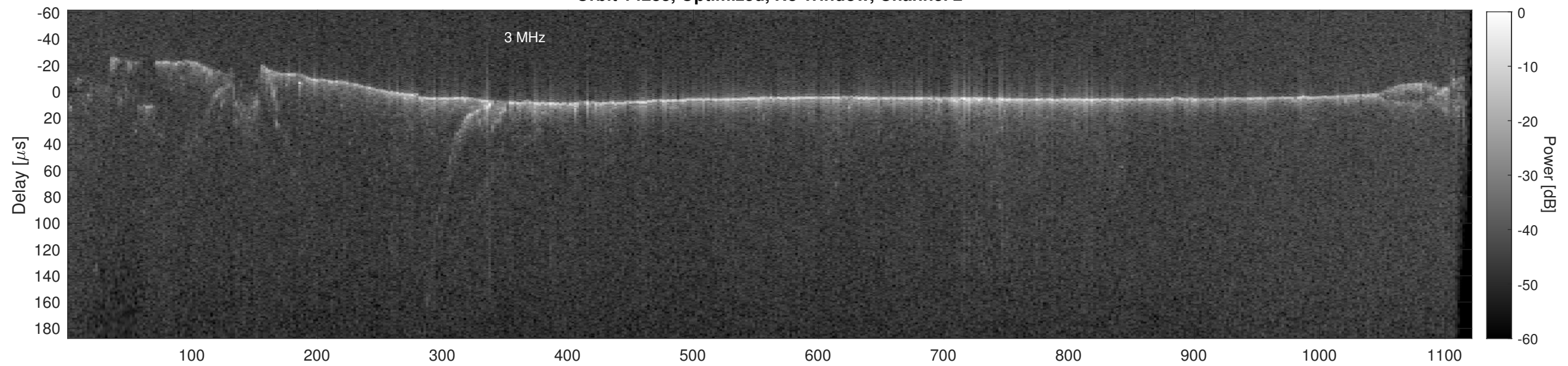
Orbit 14283, Cluttergram
