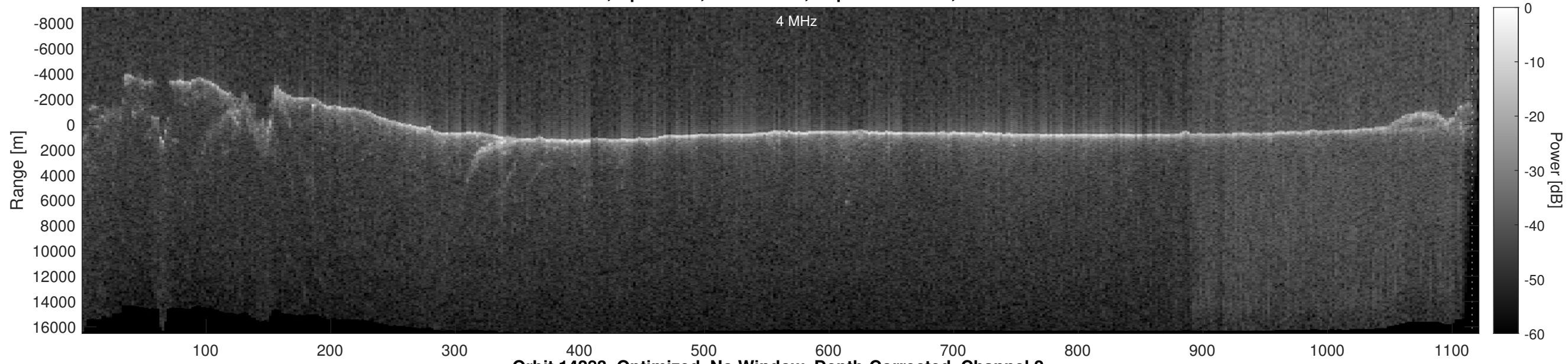
Orbit 14283, Optimized, No Window, Depth-Corrected, Channel 2
