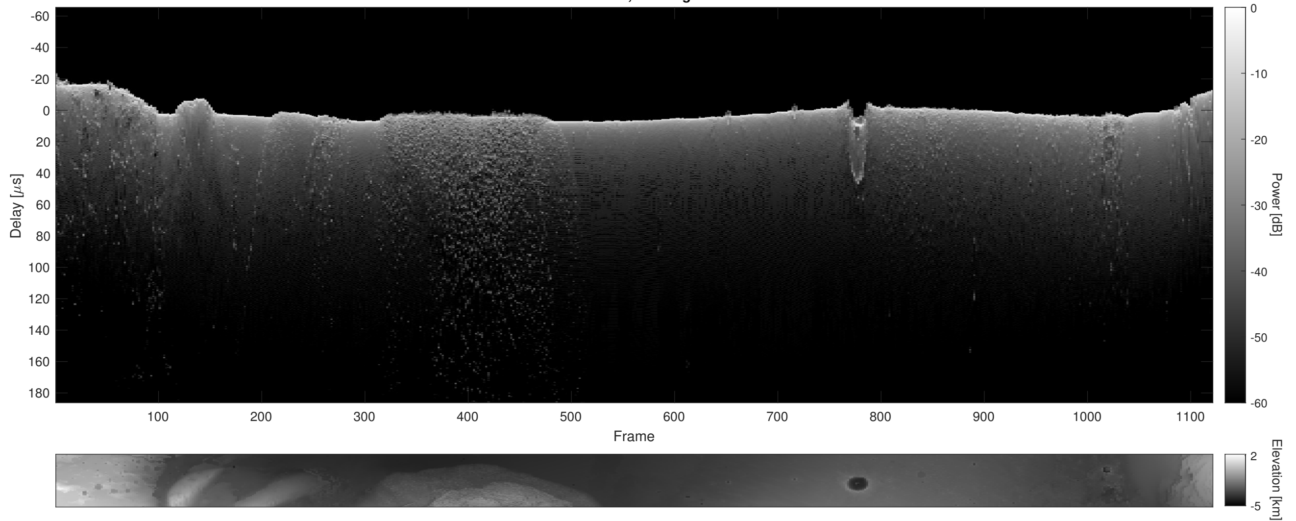
Orbit 14284, Cluttergram
