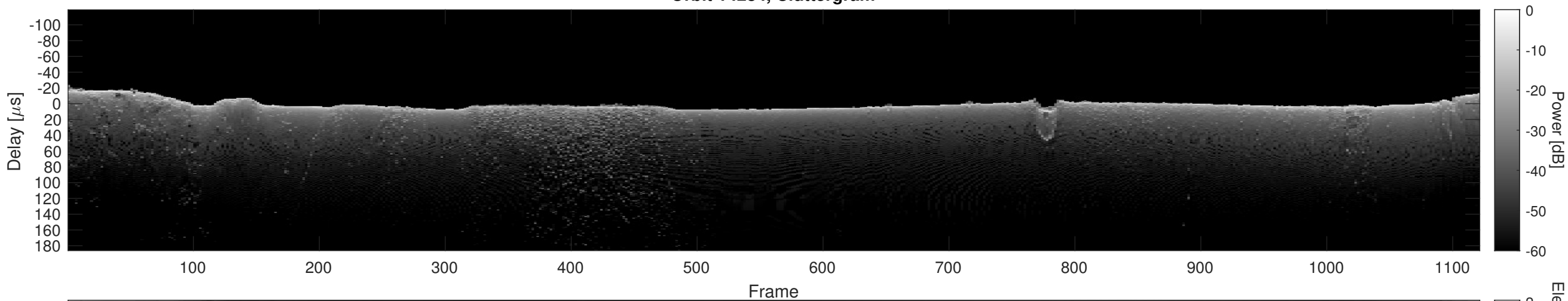
Orbit 14284, Cluttergram
