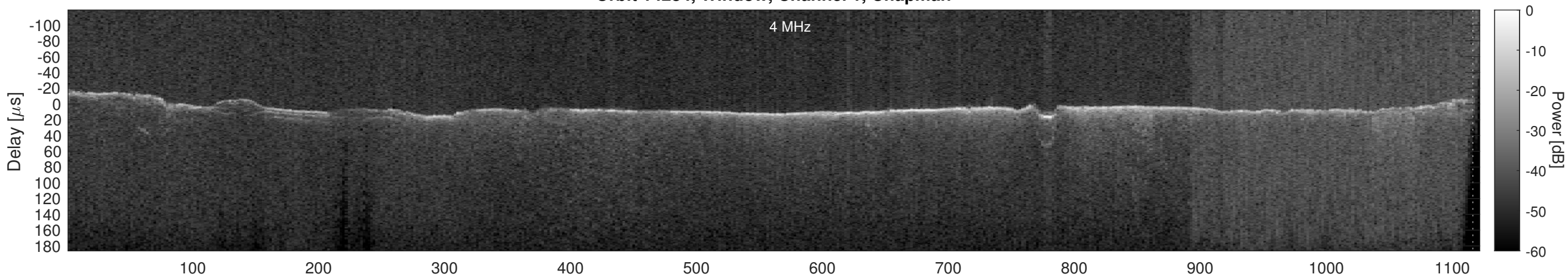
Orbit 14284, Window, Channel 1, Optimized
