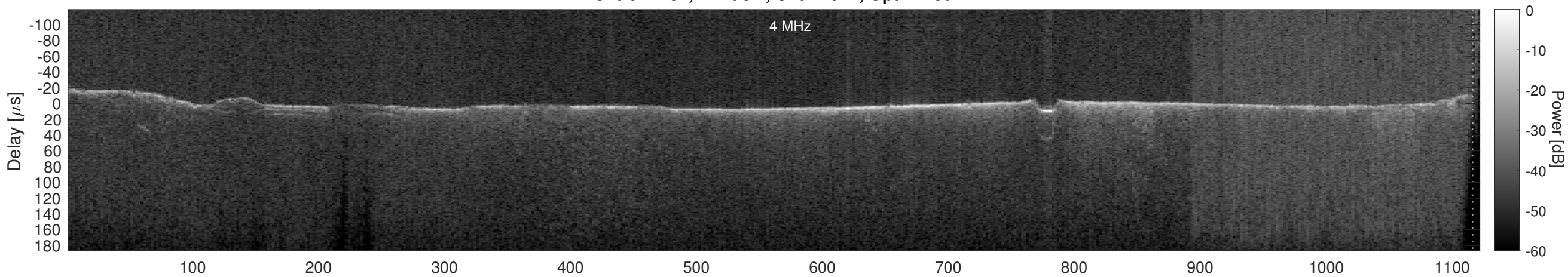
Orbit 14284, Cluttergram
