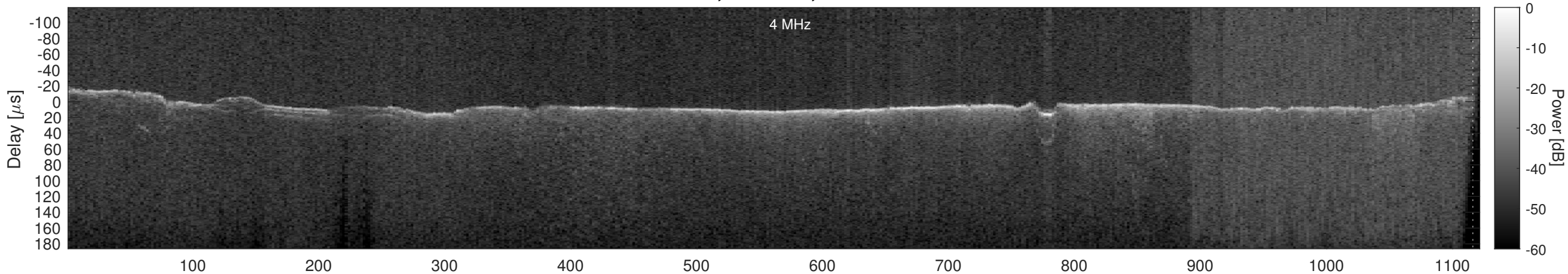
Orbit 14284, Window, Channel 1, Chapman
