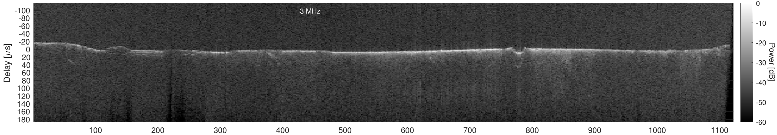
Orbit 14284, Cluttergram
