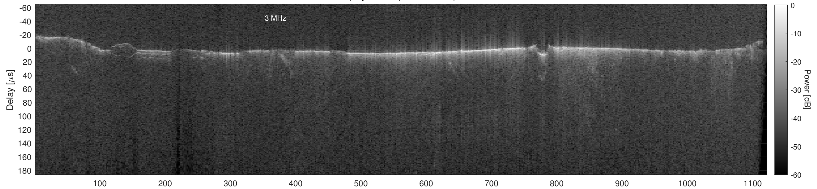
Orbit 14284, Cluttergram
