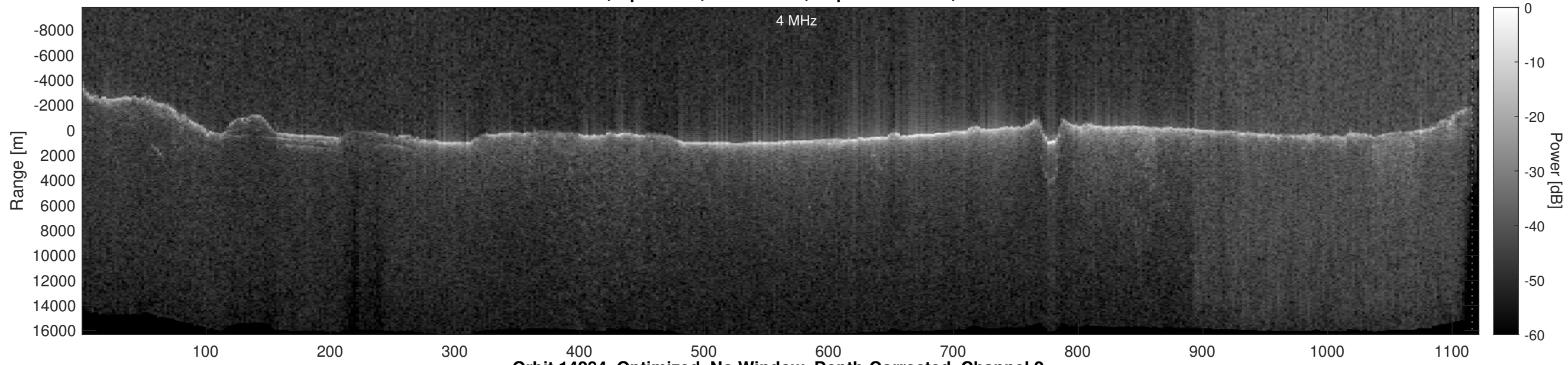
Orbit 14284, Optimized, No Window, Depth-Corrected, Channel 2
