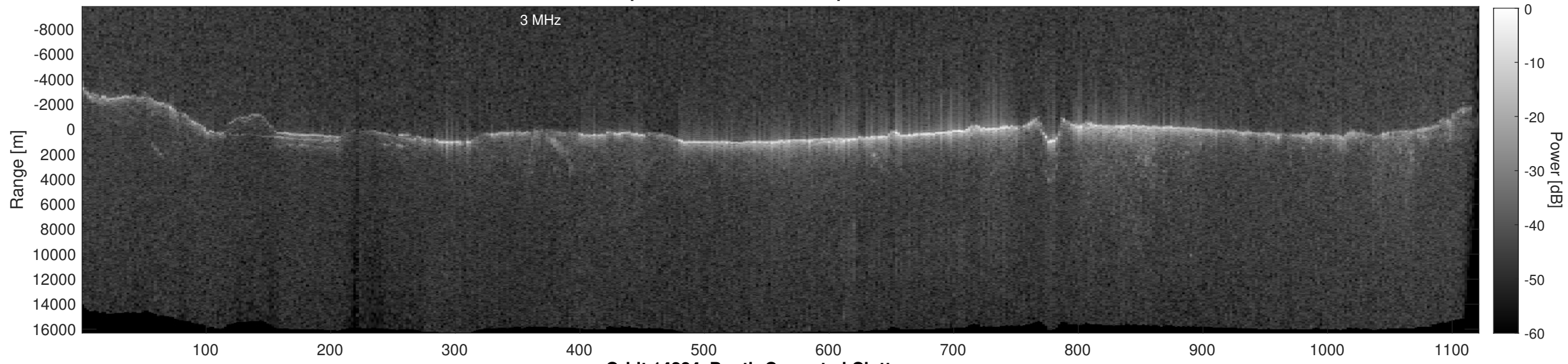
Orbit 14284, Depth-Corrected Cluttergram
