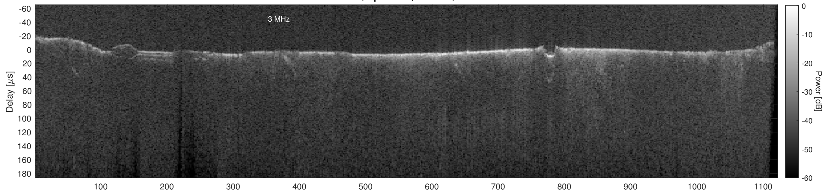
Orbit 14284, Cluttergram
