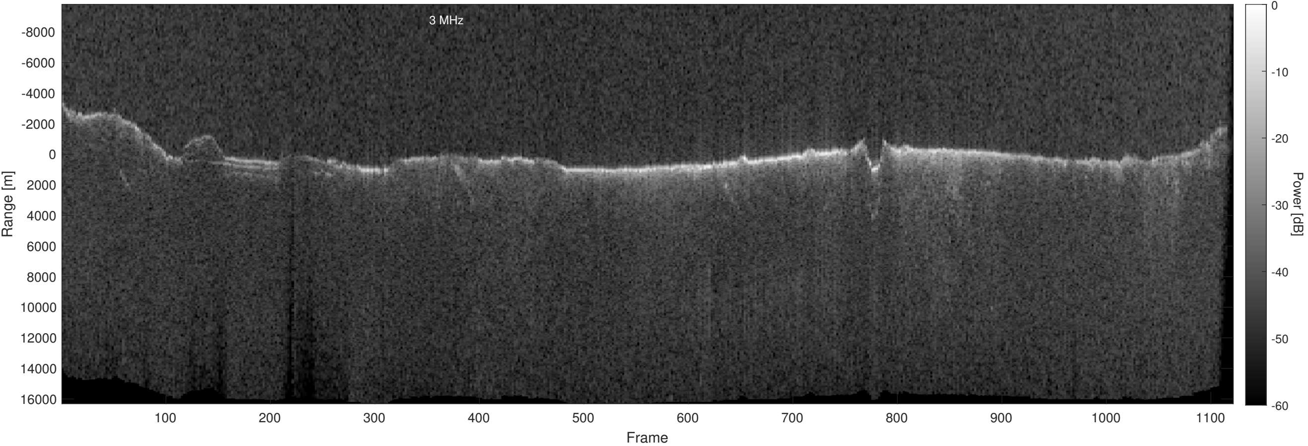
Orbit 14284, Optimized, Window, Depth-Corrected, Channel 2
