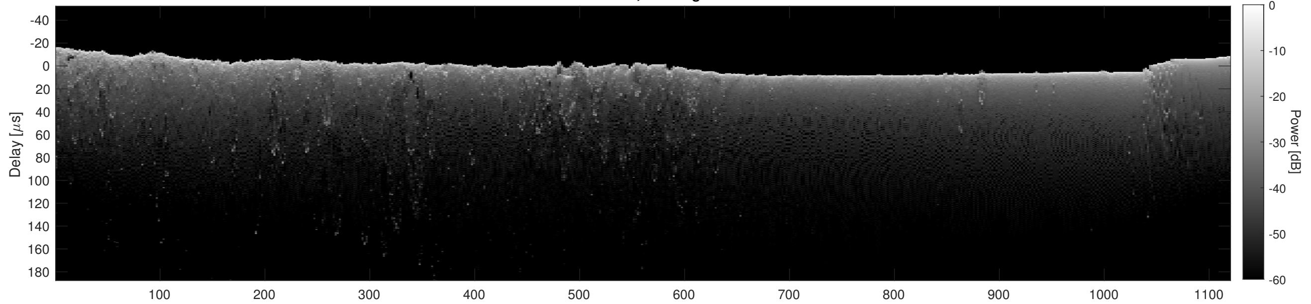
Orbit 14286, Cluttergram
