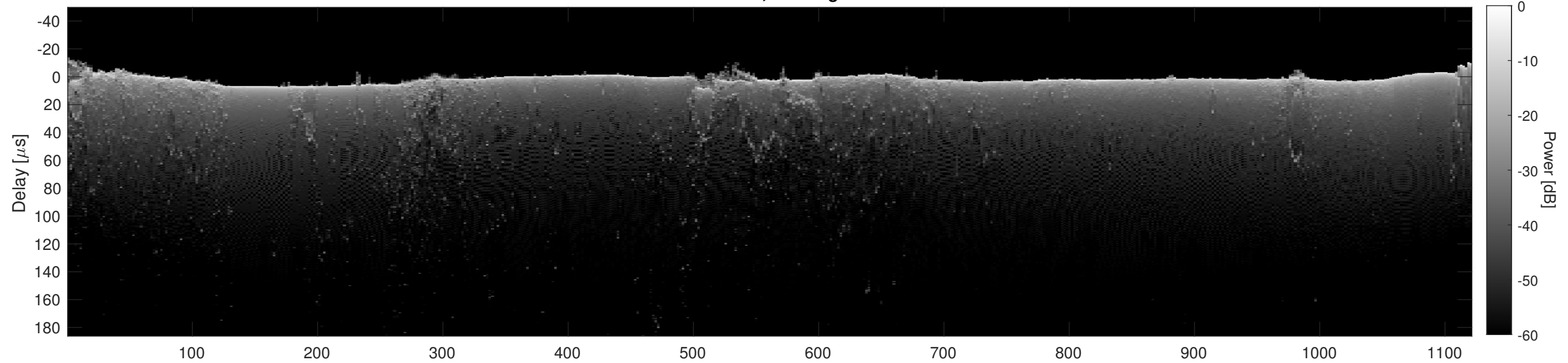
Orbit 14288, Cluttergram
