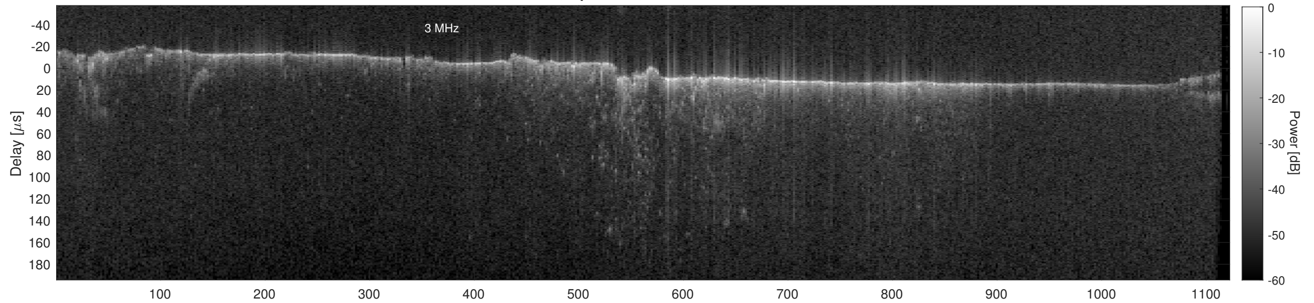
Orbit 14289, Cluttergram
