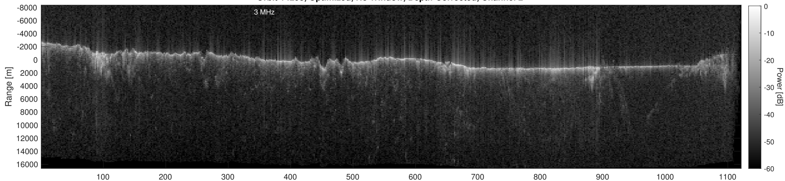
Orbit 14293, Depth-Corrected Cluttergram
