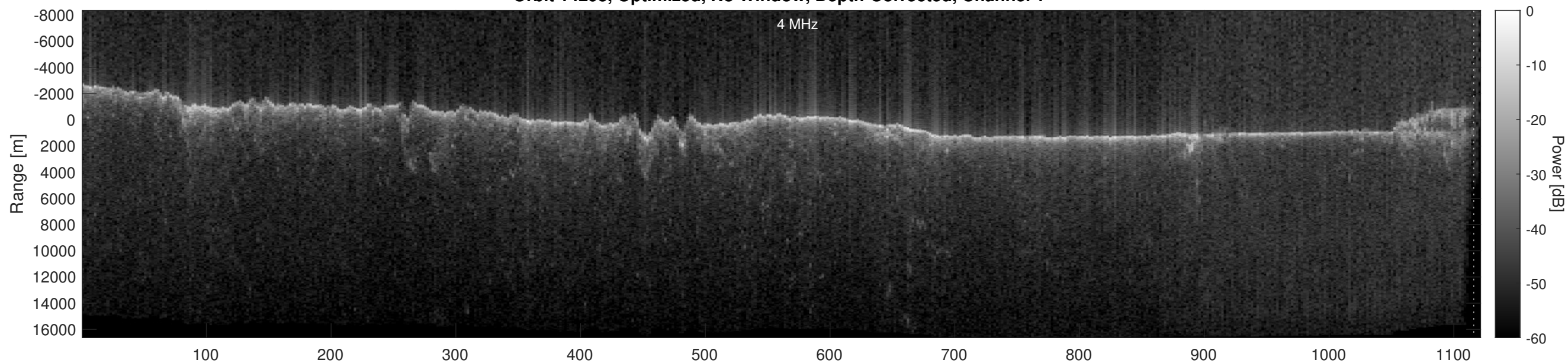
Orbit 14293, Optimized, No Window, Depth-Corrected, Channel 2
