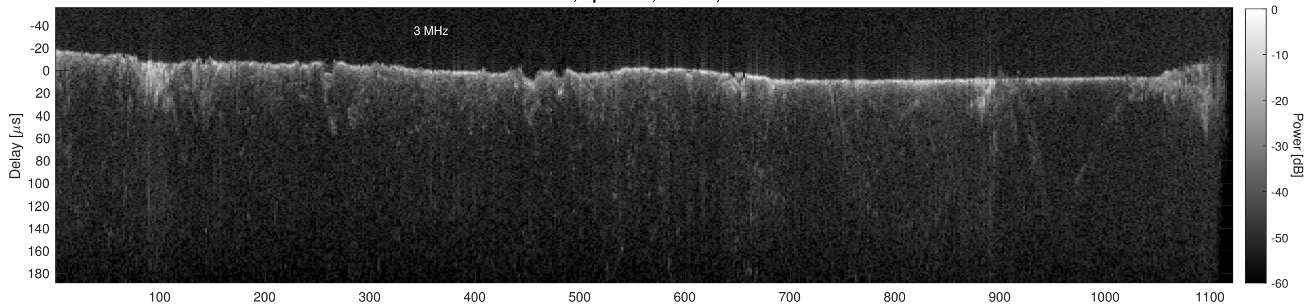
Orbit 14293, Cluttergram
