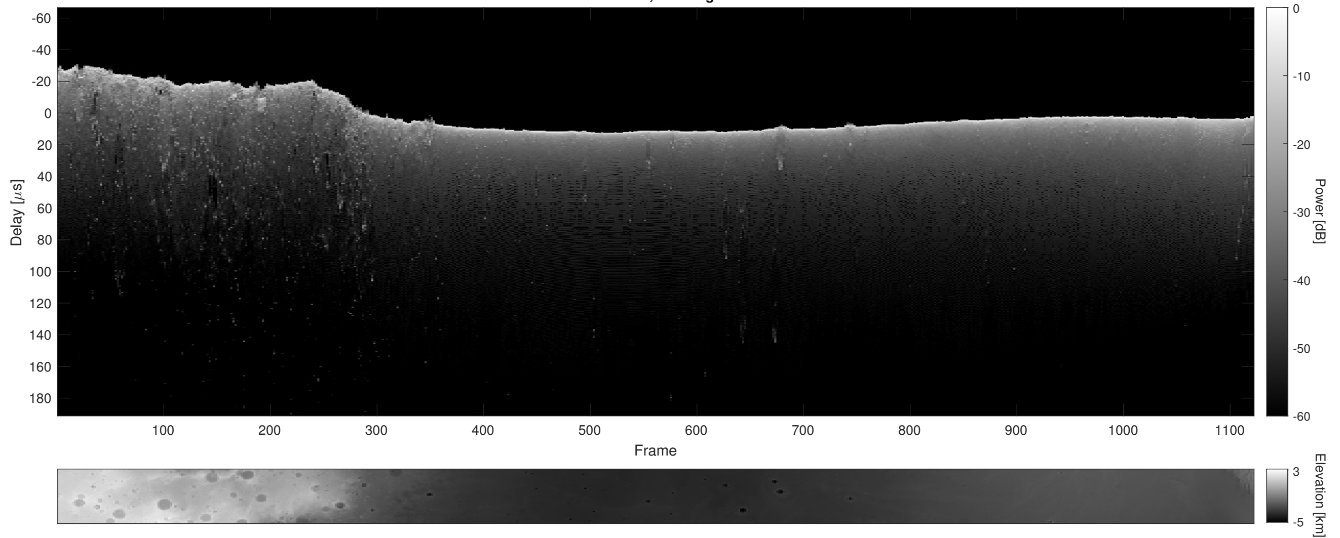
Orbit 14299, Cluttergram
