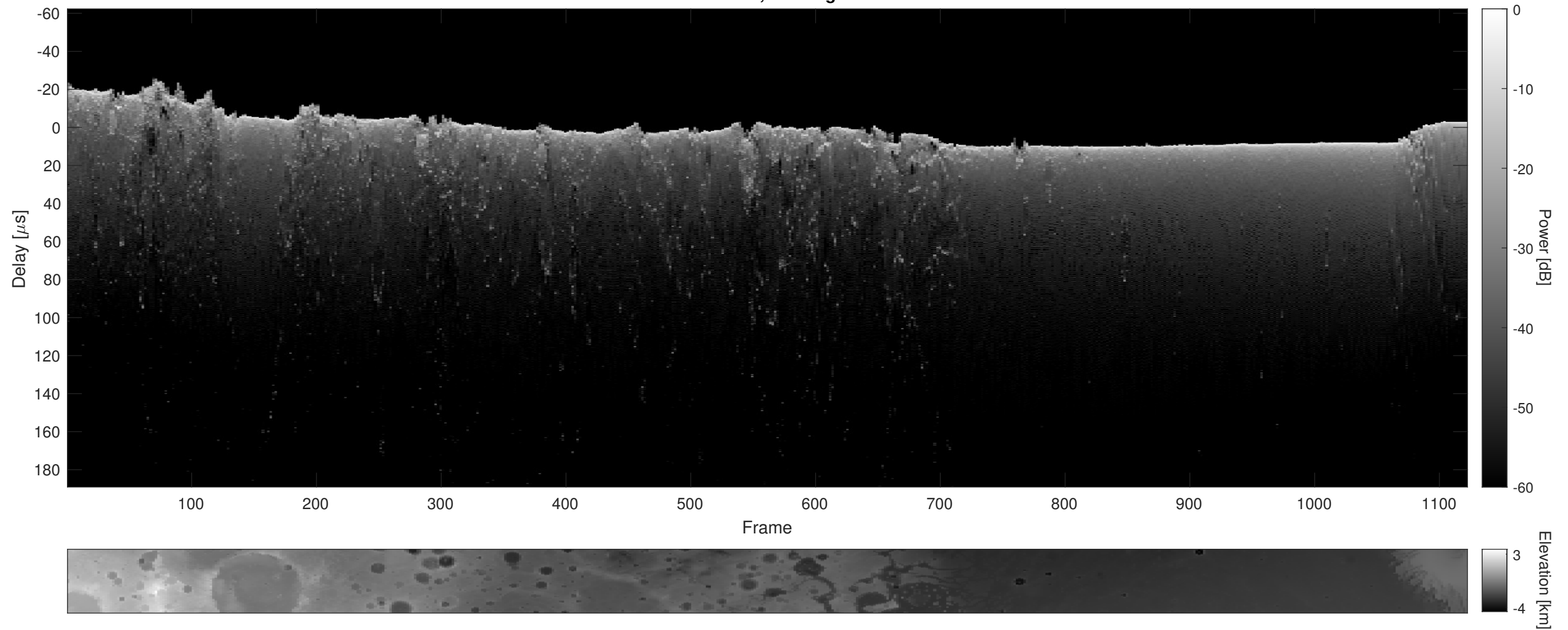
Orbit 14300, Cluttergram
