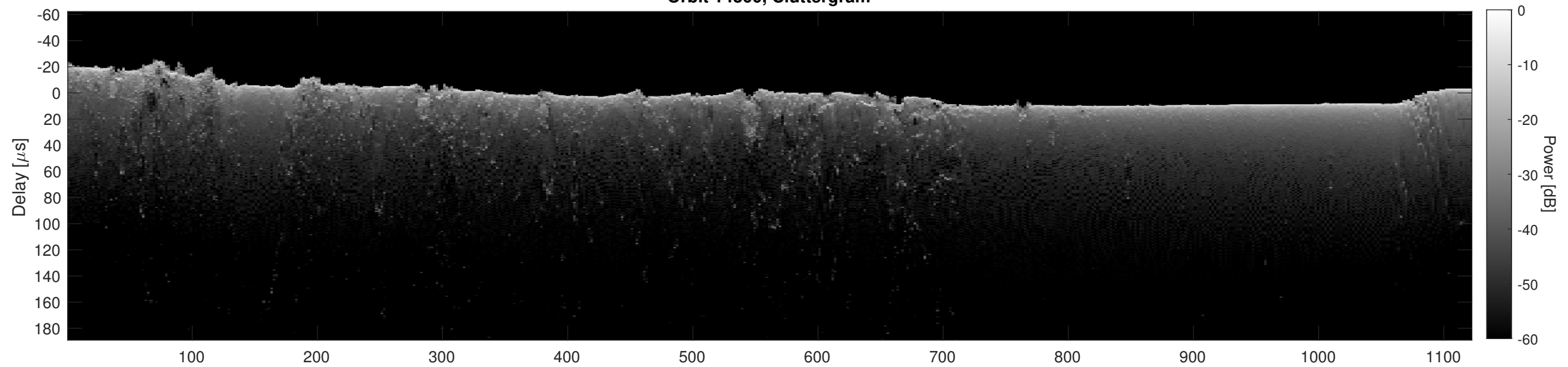
Orbit 14300, Cluttergram
