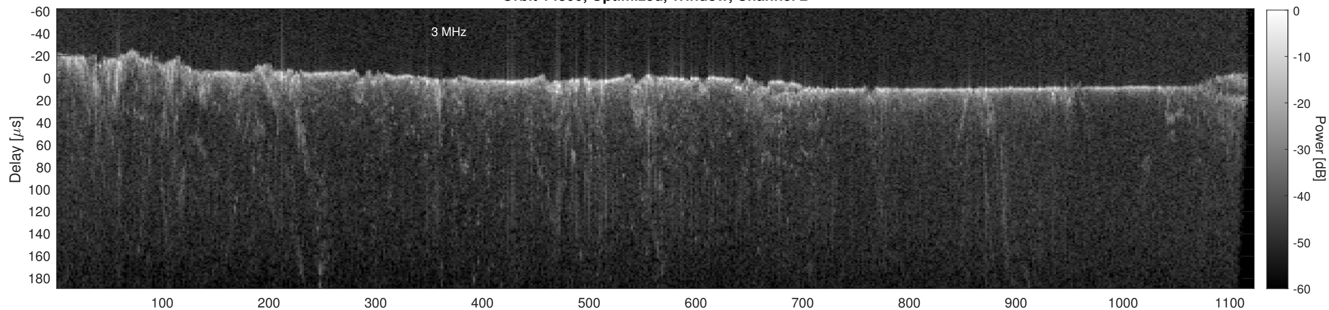
Orbit 14300, Cluttergram
