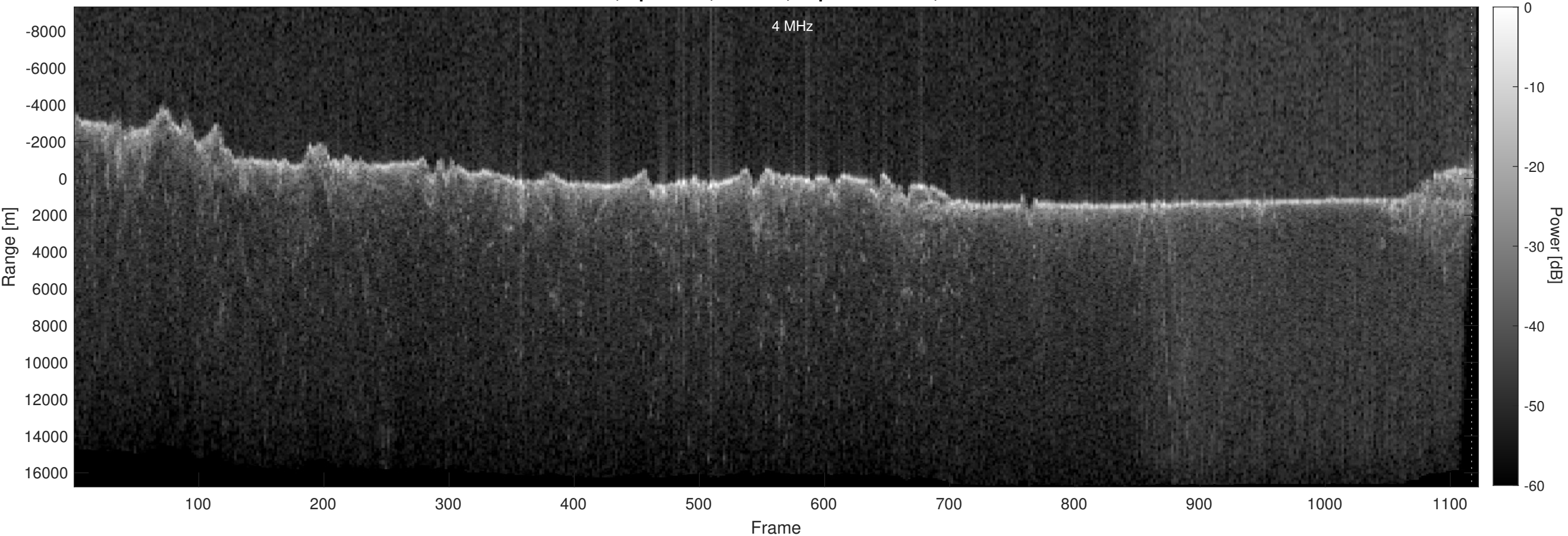
Orbit 14300, Optimized, Window, Depth-Corrected, Channel 2
