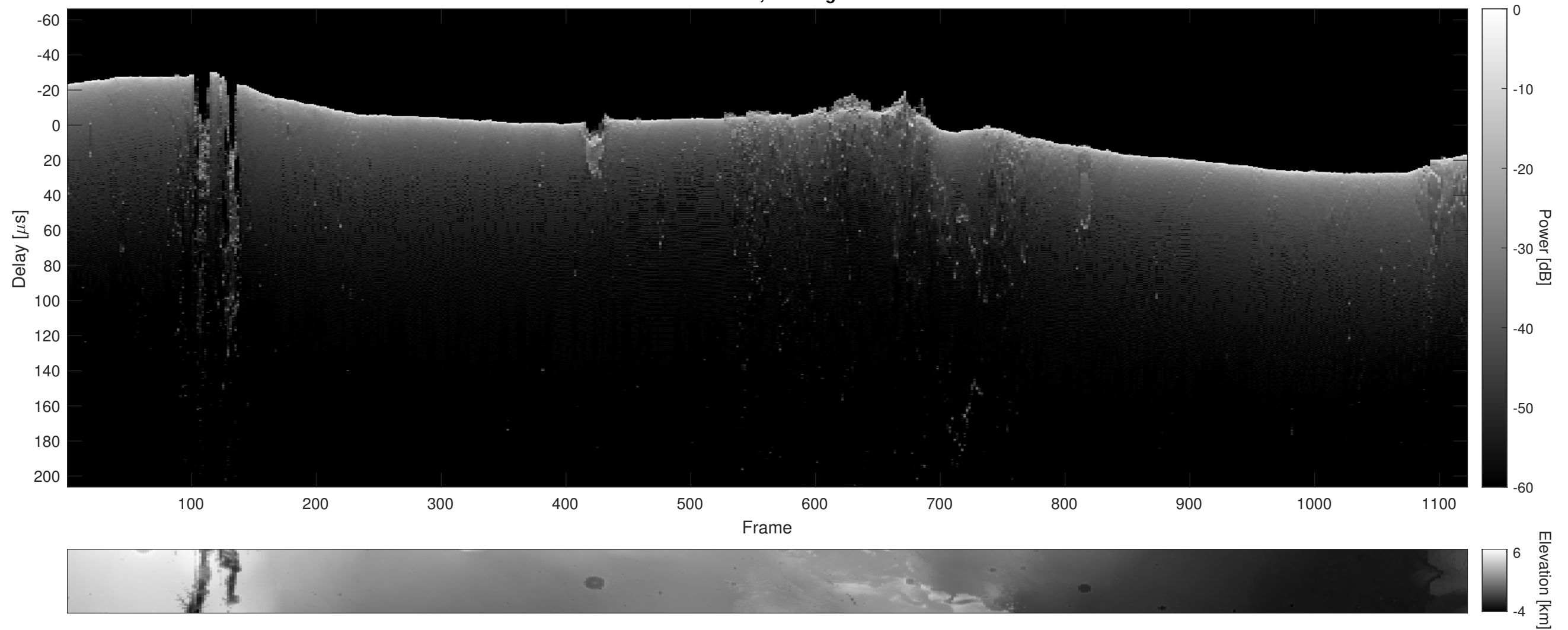
Orbit 14301, Cluttergram
