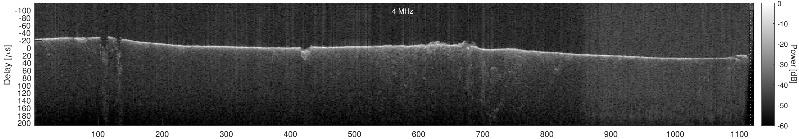
Orbit 14301, Cluttergram
