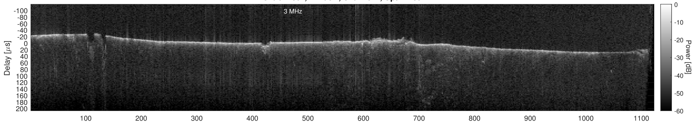
Orbit 14301, Cluttergram
