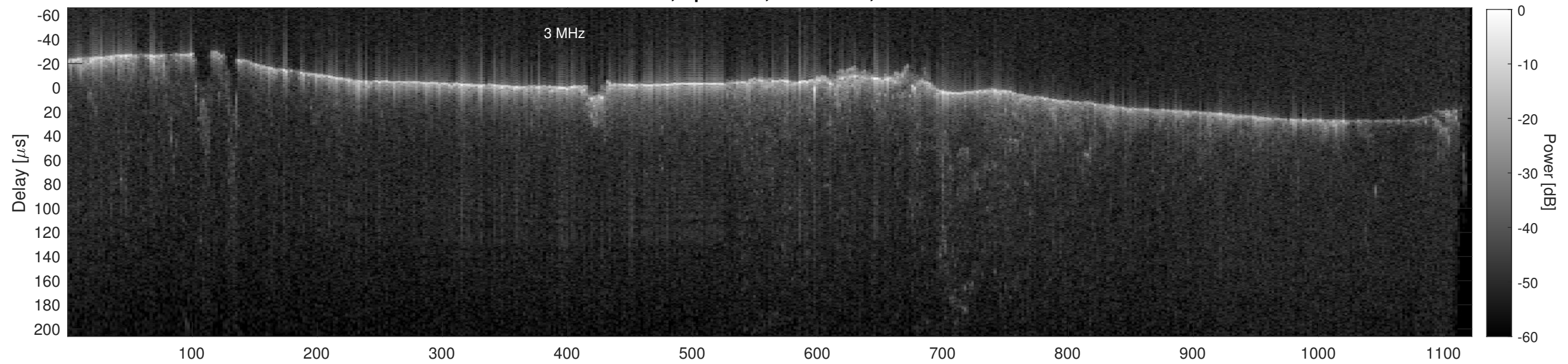
Orbit 14301, Cluttergram
