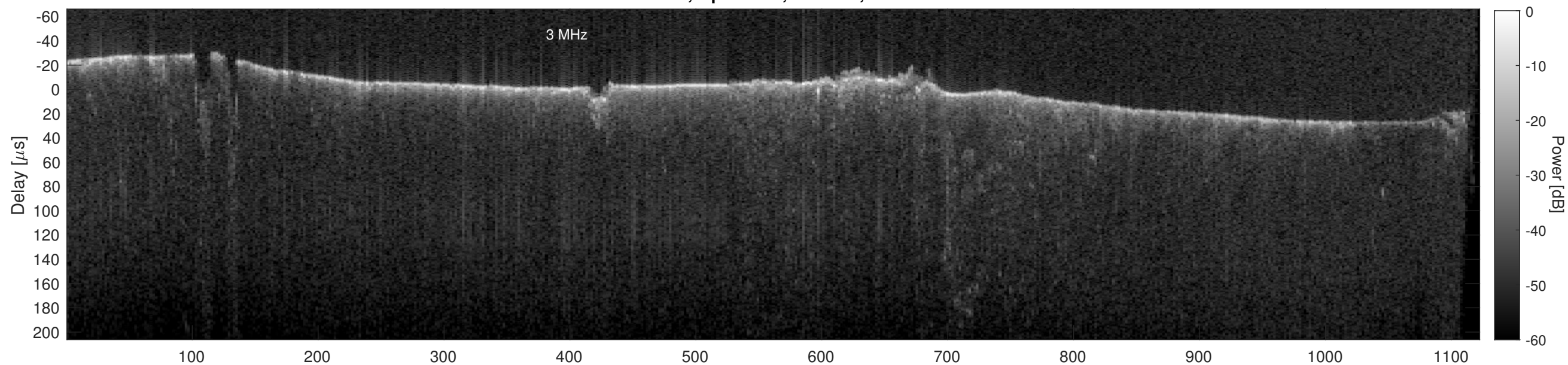
Orbit 14301, Cluttergram
