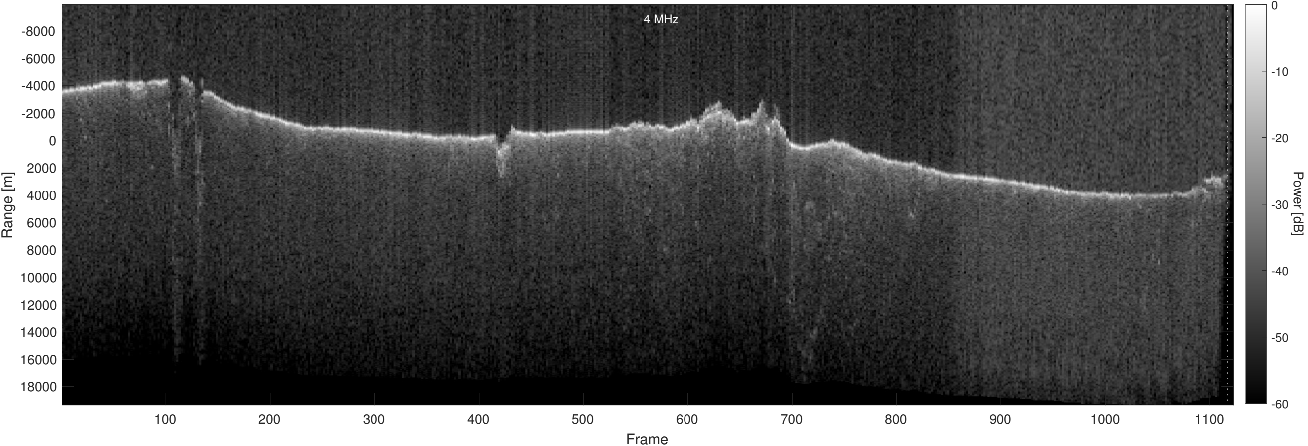
Orbit 14301, Optimized, Window, Depth-Corrected, Channel 2
