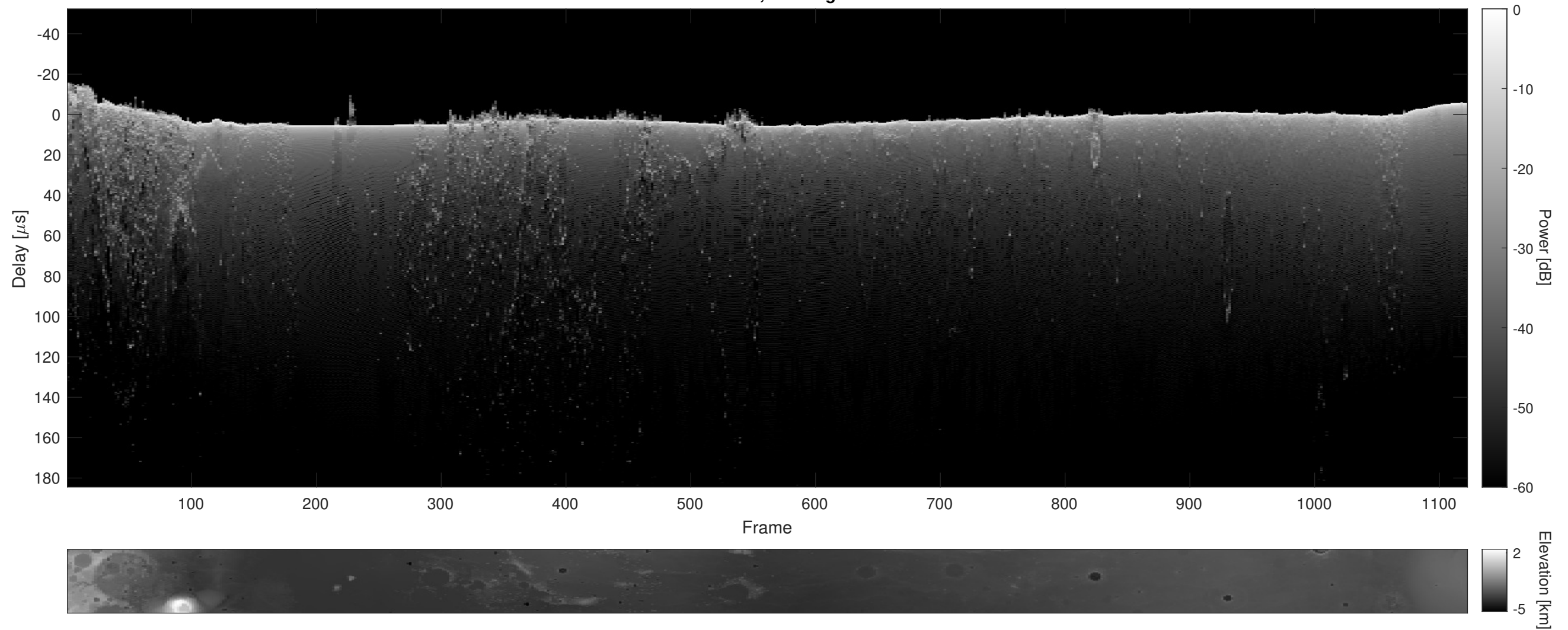
Orbit 14302, Cluttergram
