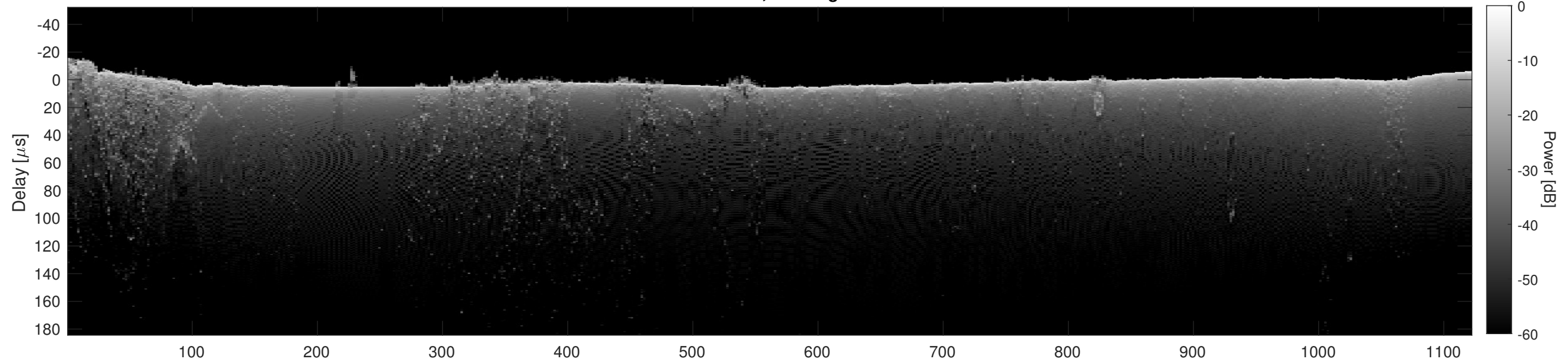
Orbit 14302, Cluttergram
