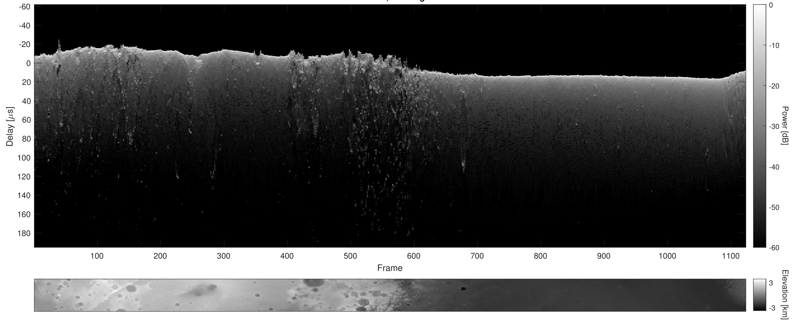
Orbit 14303, Cluttergram
