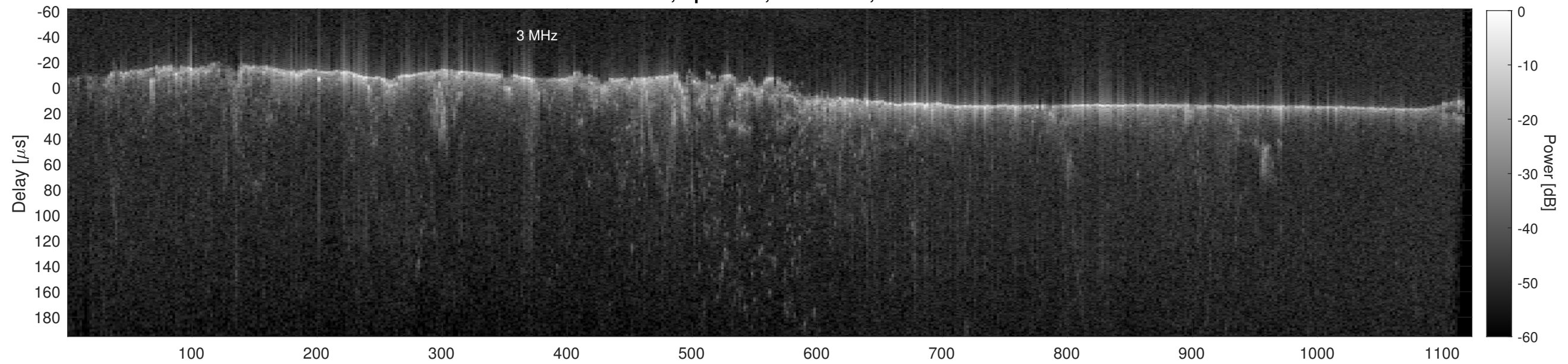
Orbit 14303, Cluttergram
